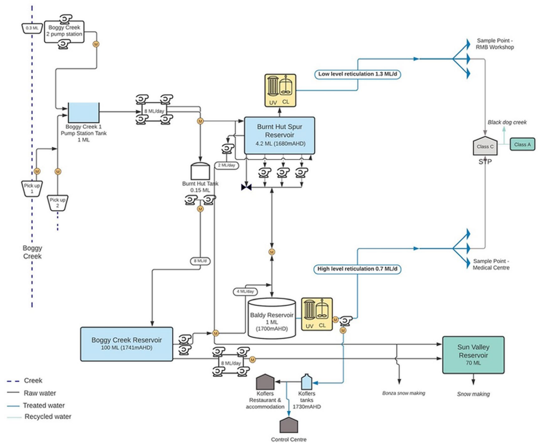
Figure 6: Mt Stirling Water Supply System
