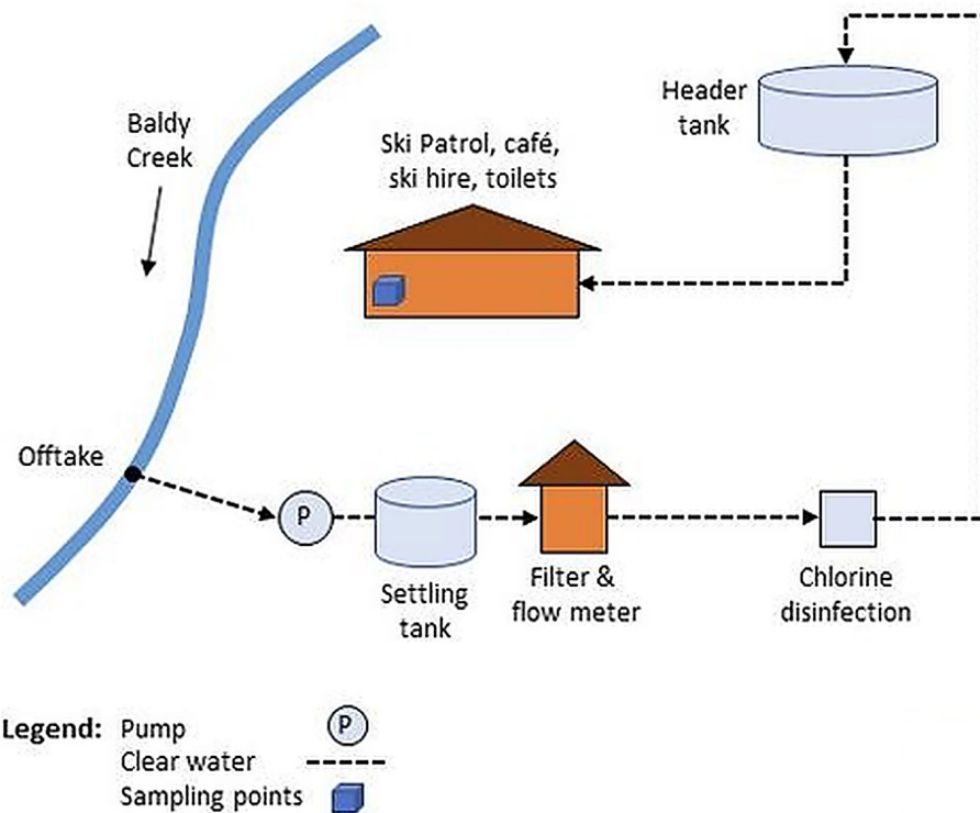
Figure 6: Mt Stirling Water Supply System
