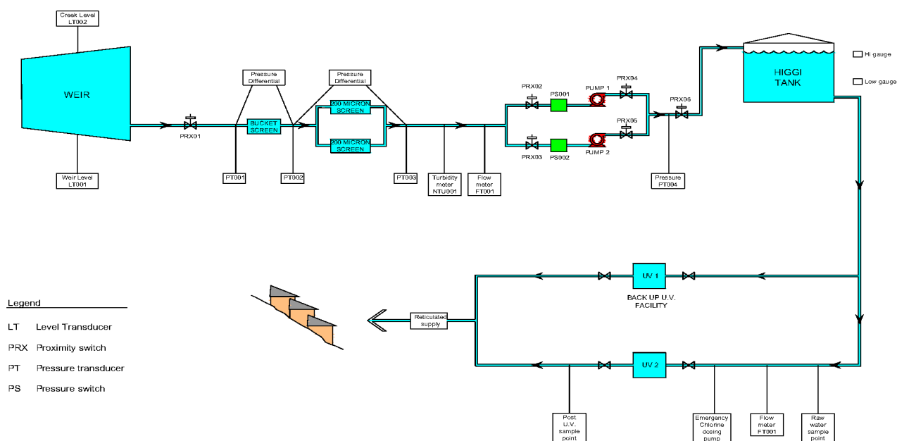
Figure 4: Mt Hotham Drinking Water Supply System
