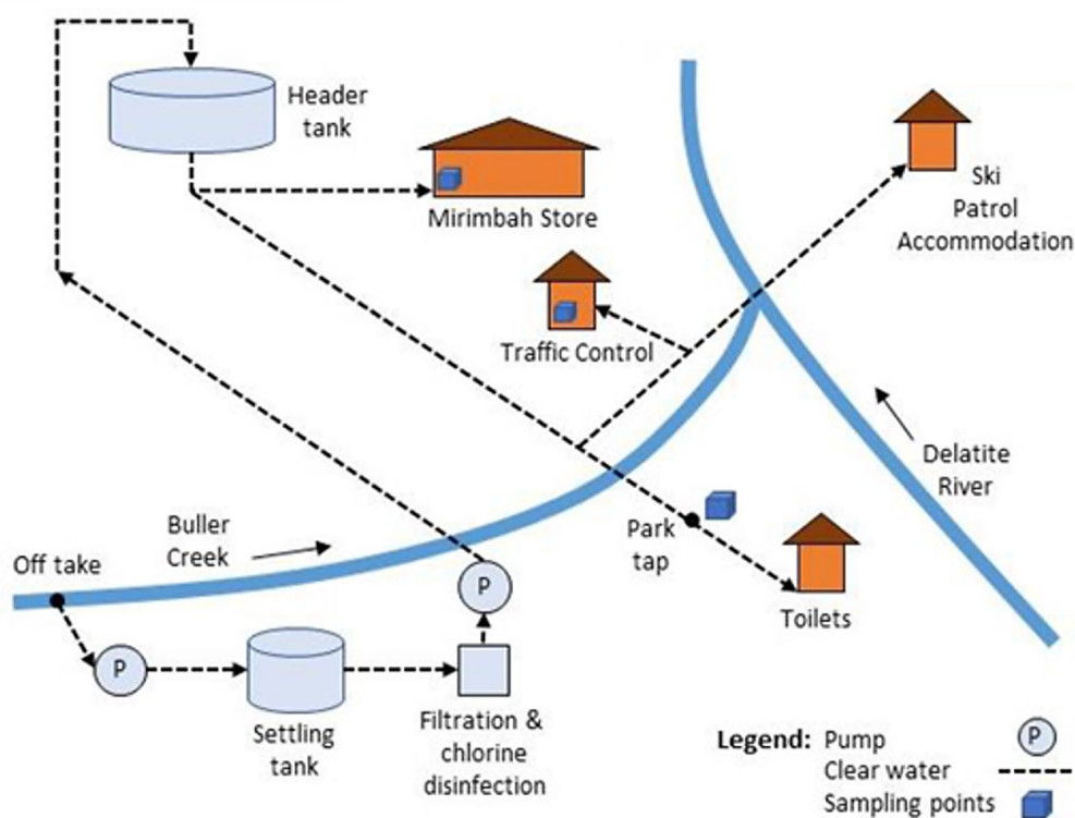
Figure 7: Mirimbah Water Supply System
