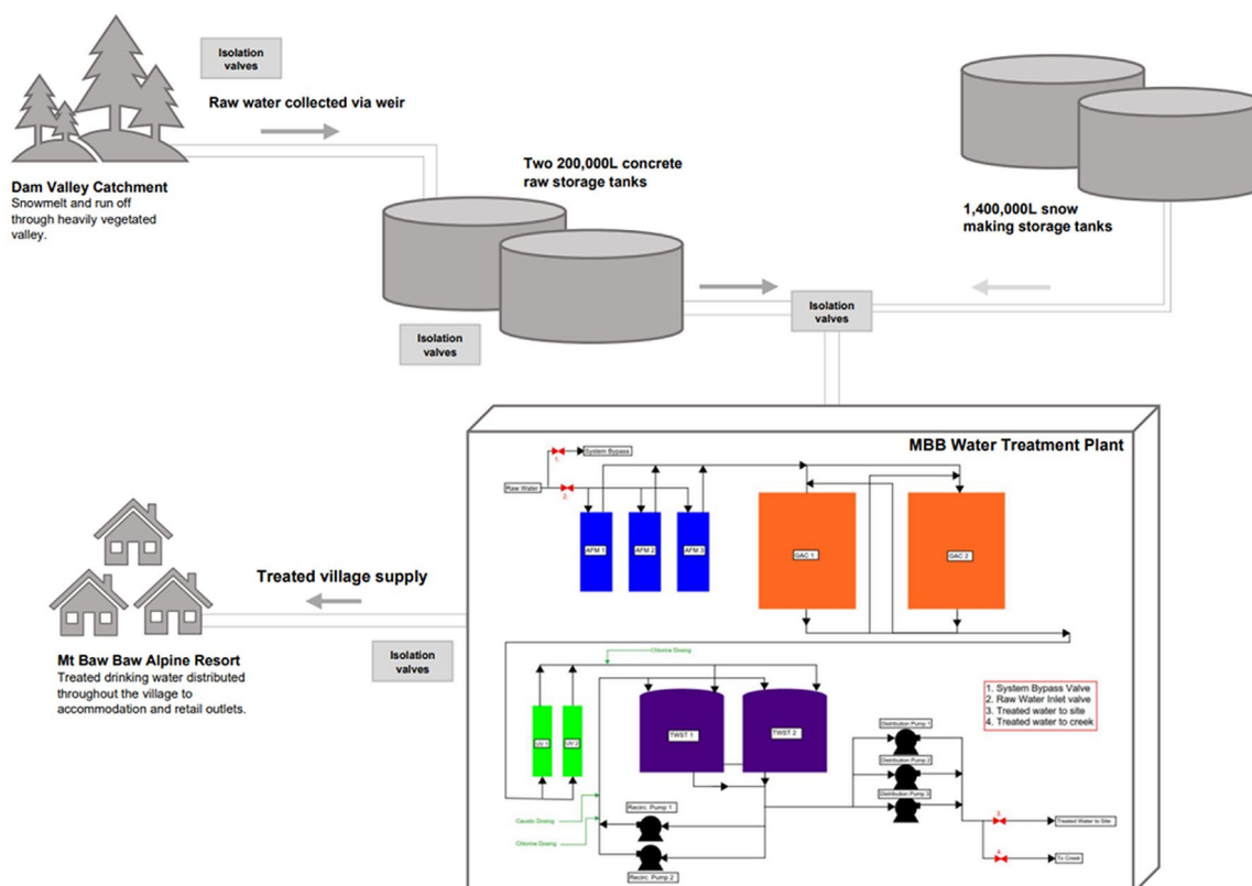
Figure 8: Mt Baw Baw Water Supply System
