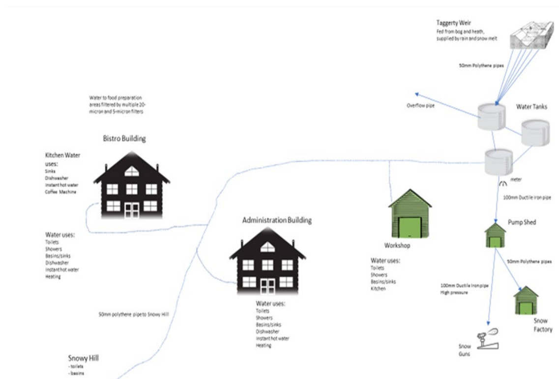
Figure 10: Lake Mountain regulated water supply system
